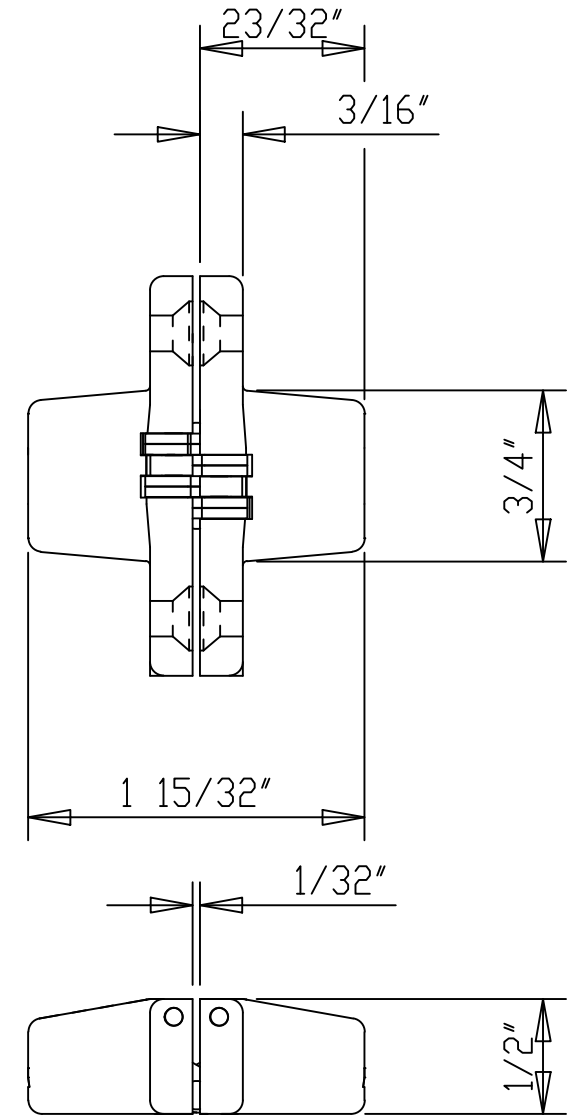
HINGE CLOSED FRONT VIEW CUT AWAY
